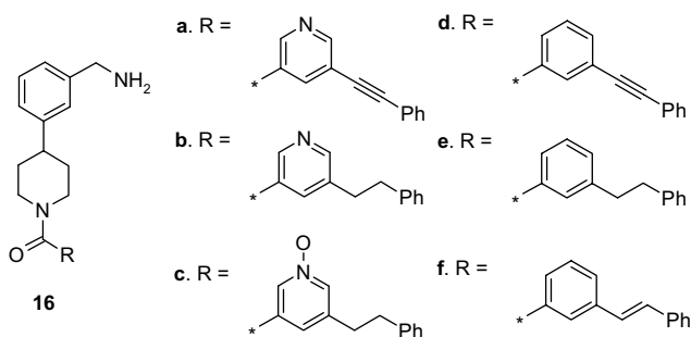
Figure 5. Compound 16a and initial analogs.
