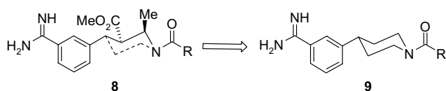
Scheme 1. \beta -Amidoester to piperidine template modification.
