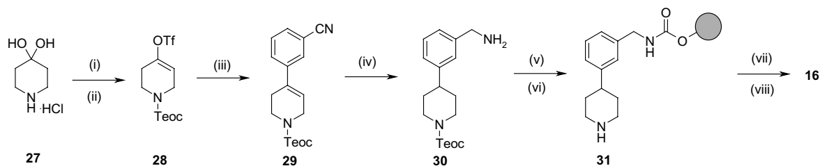
Scheme 5. Target synthesis via resin bound template (i) 2-trimethylsilylethyl- p -nitrophenylcarbonate, Et 3 N, DMAP, MeCN; (ii) Li(TMS) 2 , PhNTf 2 , THF; (iii) m -cyanophenyl boronic acid, Na 2 CO 3(aq) , LiCl, Pd(PPh 3 ) 4 , MeCN; (iv) H 2 , Pd/C, coned HCl/EtOH; (v) p -nitrophenylcarbonate Wang resin, DIEA, DMAP, DMF; (vi) TBAF, THF; (vii) RCO 2 H, DIC, HOBT, DMF; (viii) TFA, DCM.
