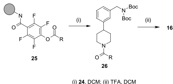
Scheme 4. Target synthesis via TFP-resin loaded carboxylic acids.
