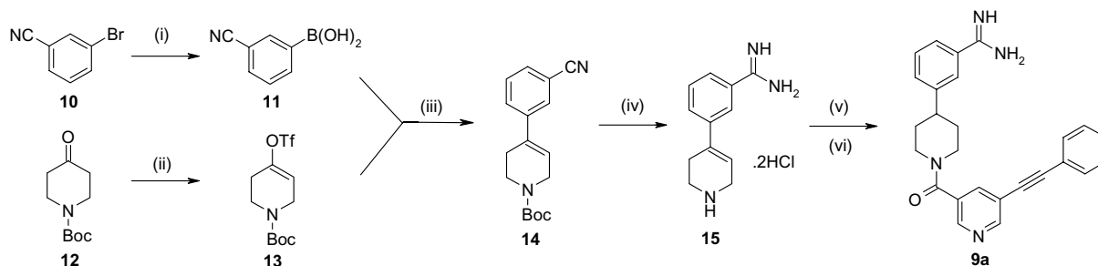
Scheme 2. Synthesis of benzamidinepiperidine template and subsequent coupling. Reagents and conditions: (i) a. n -BuLi, B(OCHMe) 2 , THF, b. aq HCl; (ii) LDA, PhNTf 2 , THF; (iii) (Ph 3 P) 4 Pd, Na 2 CO 3 , MeCN/H 2 O; (iv) a. MeOH–HCl, b. MeOH–NH 3 ; (v) 5% Pd/C, H 2 , MeOH; (vi) Et 3 N, TBTU, 3-phenylethynyl-pyridinecarboxylic acid, DMF.
